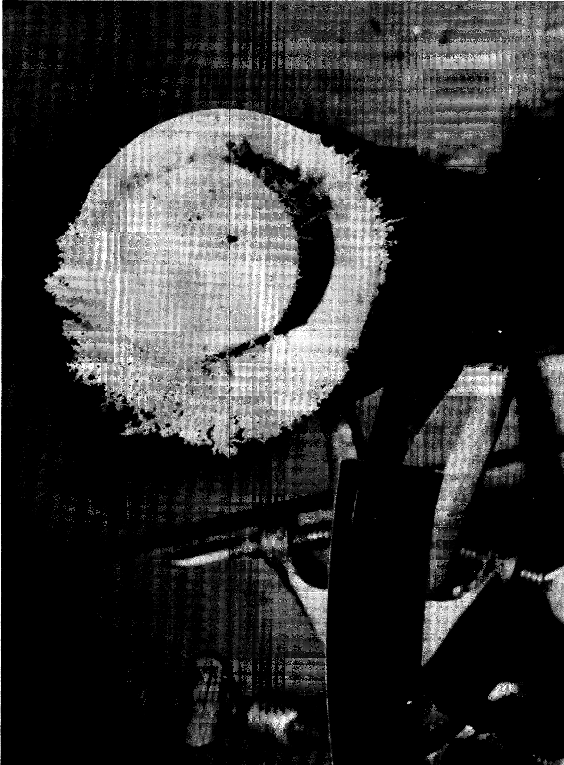
Fig 16 Formation of Ammonium Nitrate on Top of Irradiation Explosion Proof Capsule Containing Lead Azide. Subjected to a 1.16 \times 10^9 R Gamma Dose (Refs 254 & 257)
